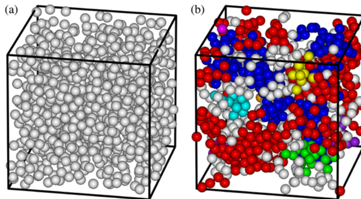
Figure 2. Simulation snapshots of N = 864 particles at a volume fraction of \eta = 0.164 . (a) ordinary hard spheres; (b) adhesive hard spheres at \tau = 0.13 . The largest clusters have been shaded differently. The largest cluster (red, online version) percolates.
