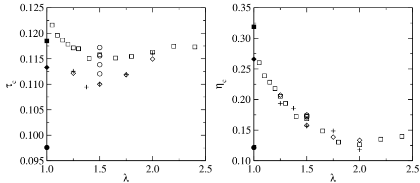
Figure 1. The critical effective temperature \tau_c (left) and volume fraction \eta_c (right) of square well fluids with range parameter \lambda . Open symbols are taken from [18] (circles), [19] (squares), [20] (diamonds) and [21] (plus signs). Filled symbols at \lambda = 1 are the adhesive hard sphere limits from the Percus–Yevick compressibility (circles) and energy (squares) routes, and from simulation (diamonds).
