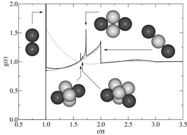
Figure 3. The radial distribution function, g(r) , at a volume fraction of \eta = 0.164 as for figure 2. Solid curve: adhesive hard spheres at \tau = 0.13 from simulation; dashed curve: the corresponding Percus–Yevick prediction; dotted curve: hard spheres. Physical clusters contributing to certain features of the solid line are indicated.
