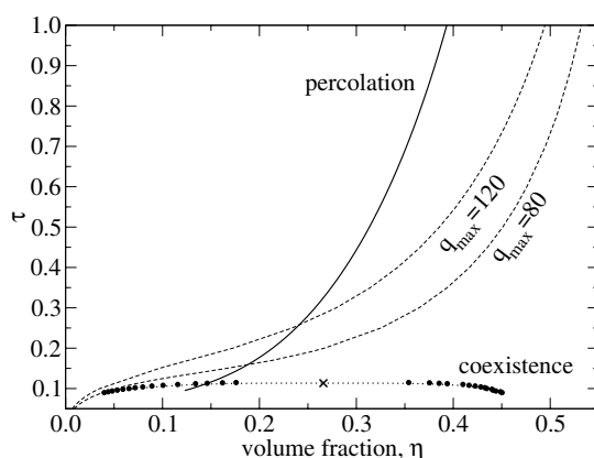
Figure 7. The phase diagram of adhesive spheres in the \eta – \tau plane. The dotted curve with circles is the fluid–fluid coexistence curve from simulation, with the critical point marked by a cross [13]. The solid curve is the percolation threshold from simulation [14] to the high \eta side of which infinite clusters exist in the system. The dashed curves are the mode-coupling attractive glass transition with cut-offs \sigma q_{\max} = 80 and 120 as marked. Mode-coupling theory predicts structural arrest to the high \eta side of this threshold.
