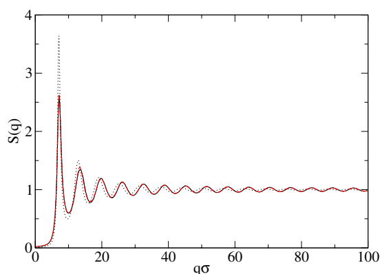
Figure 6. The static structure factor of adhesive hard spheres at \tau = 1.32 and \eta = 0.52 , illustrating its slowly decaying 1/q tail. The solid curve is from simulation and the dashed curve (red, online version) from Percus–Yeick theory. These two lines are barely discernable. For comparison, the dotted curve shows the simulation result for ordinary hard spheres at the same volume fraction.
