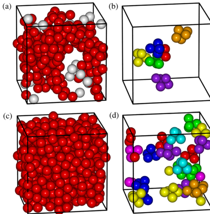
Figure 5. Snapshots from grand canonical simulations [14] at \tau = 0.13 . All particles are shown in the left-hand frames, with particles in the percolating cluster darkly shaded (red, online version). On the right, any particles not belonging to a rigid subunit have been removed, and different shades are used to distinguish between the subunits. Frames (a) and (b) are taken from simulations with an average packing fraction of 0.17, and (c) and (d) for an average of 0.50.
