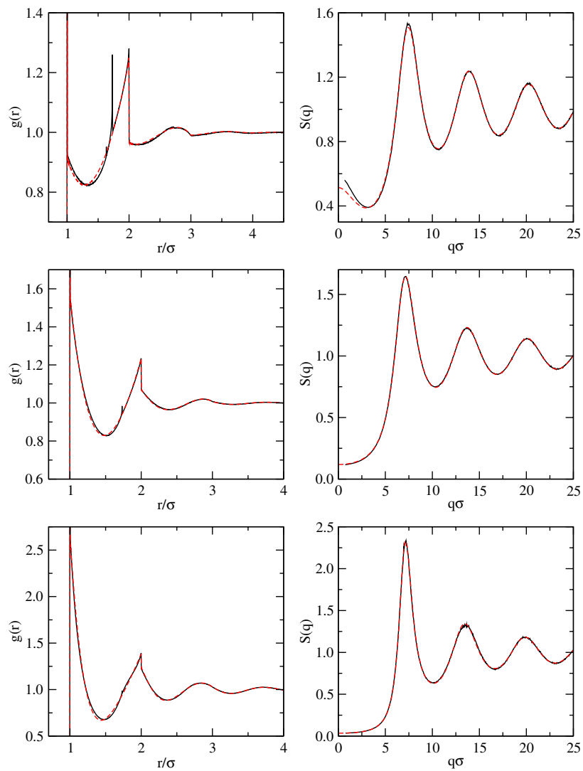
Figure 4. The radial distribution function (left) and the static structure factor (right) under three sets of conditions: \tau = 0.2 , \eta = 0.32 (top row); \tau = 0.5 , \eta = 0.4 (middle row); \tau = 1 , \eta = 0.5 (bottom row). Solid curves are from simulation and dashed curves (red, online version) from Percus–Yevick theory. The lines are not always distinguishable from each other.
